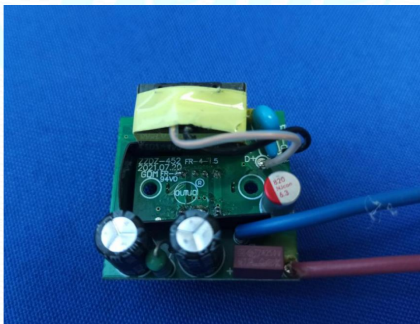
Figure 4 PCB View
