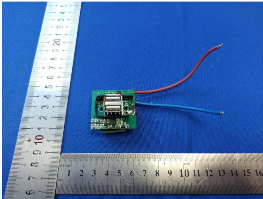
Figure 3 PCB View
